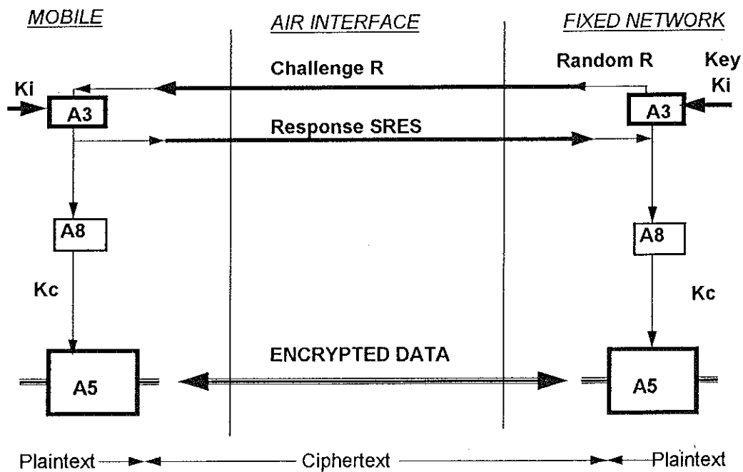
Figure 1. Encryption for GSM
